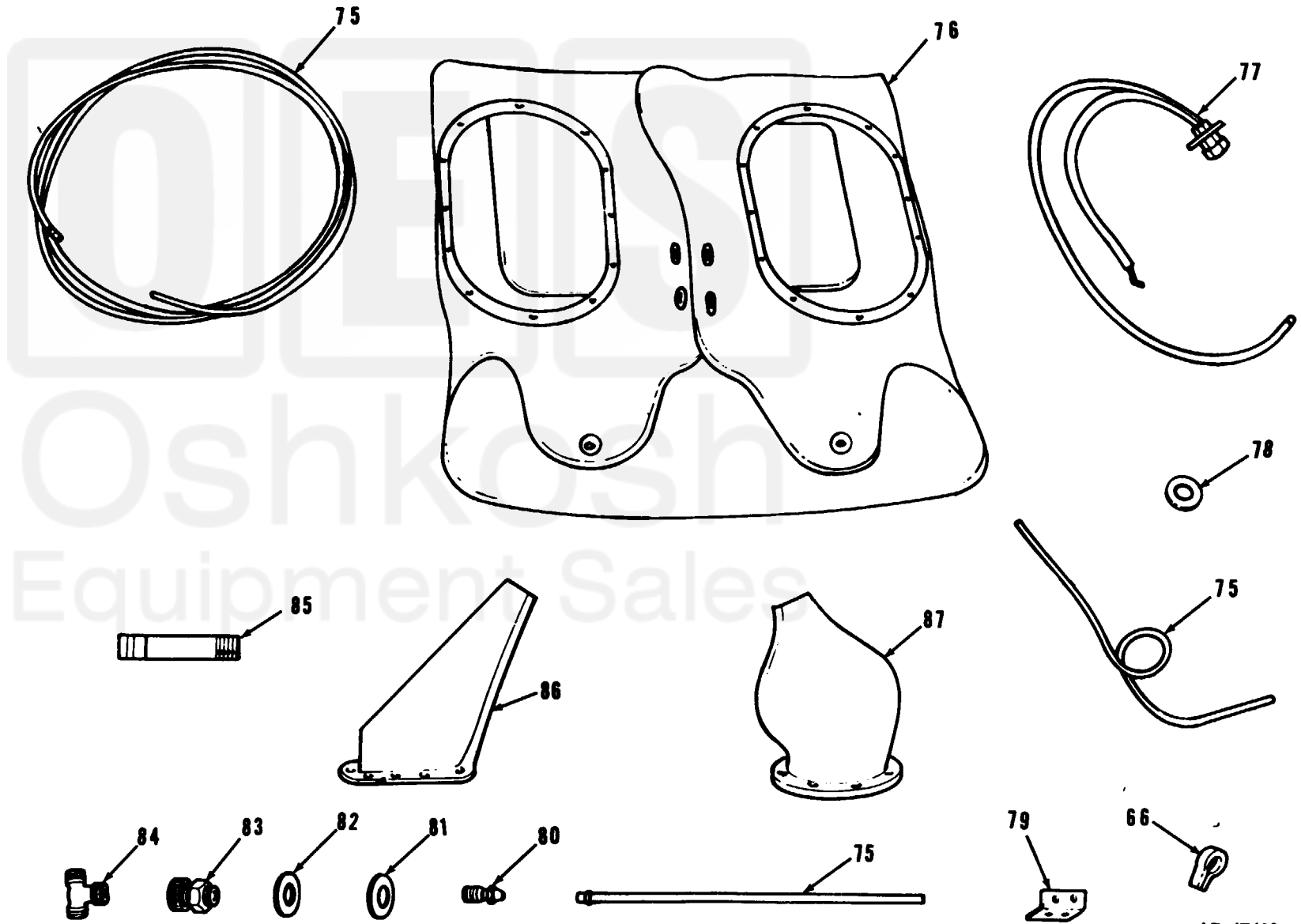
Figure 303. Multifuel personnel heater (4 of 4).
